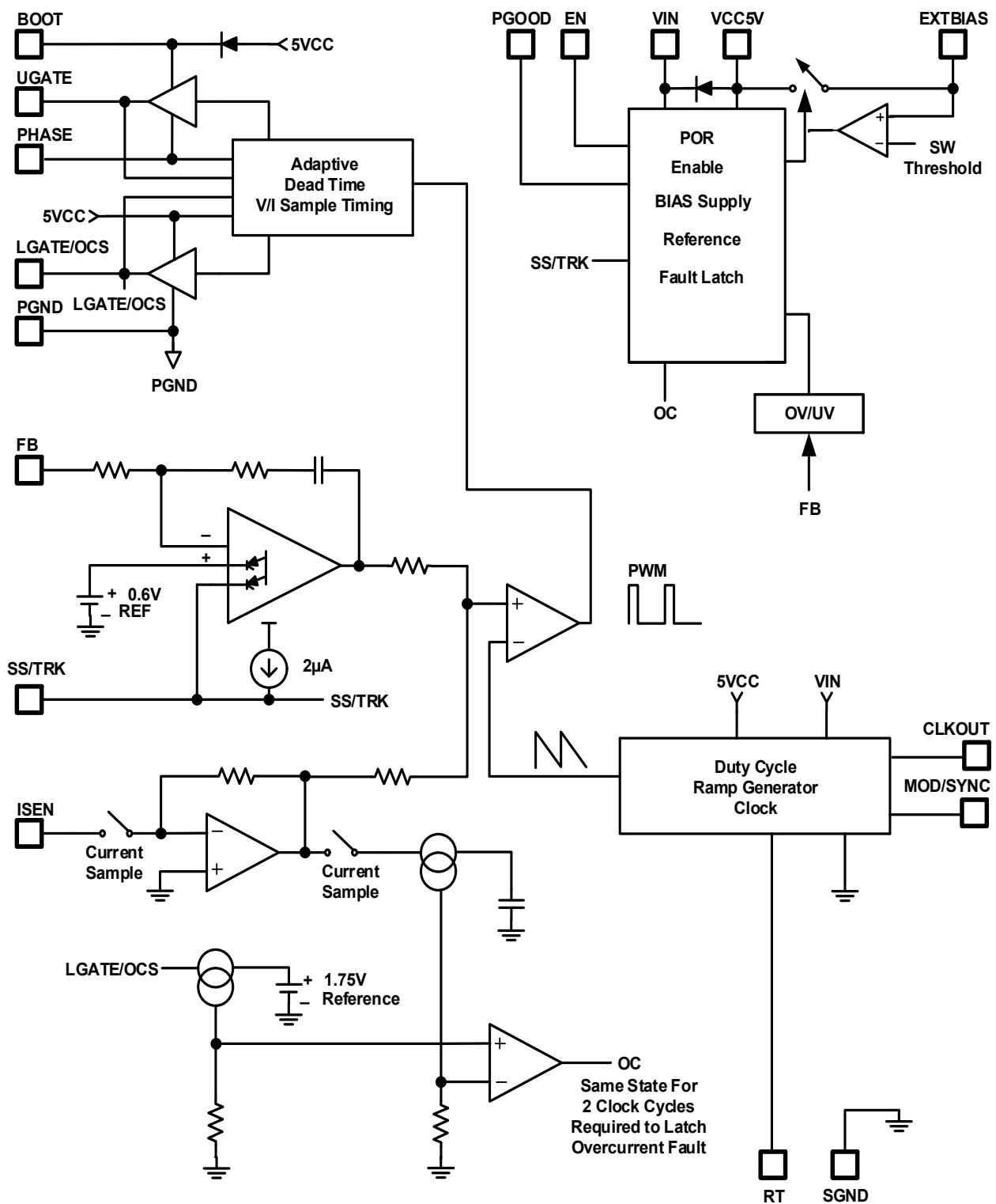
Figure 3. Block Diagram
