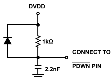
FIGURE 14. \overline{\text{PDWN}} DELAY CIRCUIT
