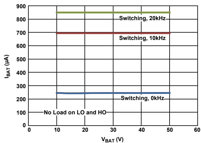
Figure 14. HIP2104 V_{BAT} Operating Current
