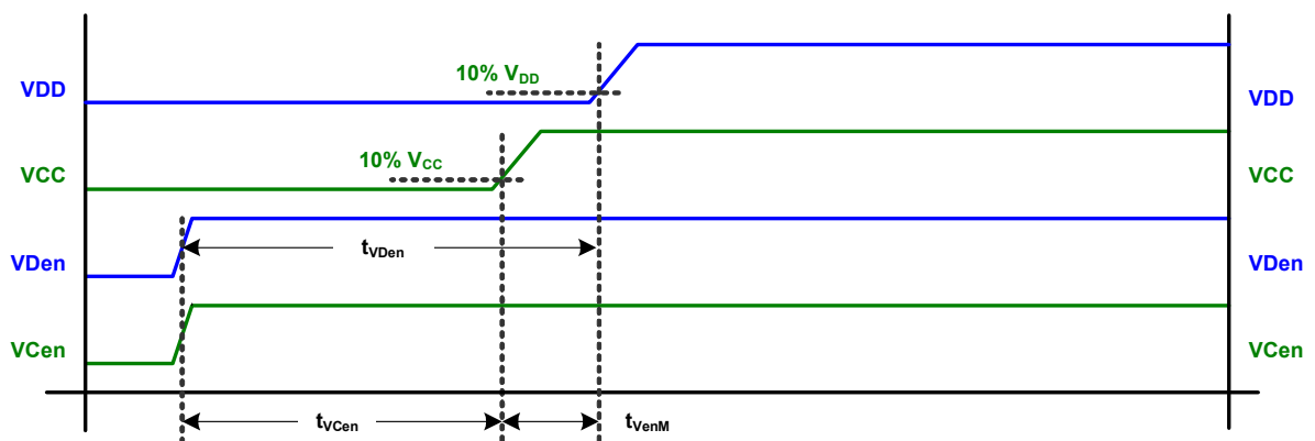
Figure 8. VCCen and VDen Delay Matching
