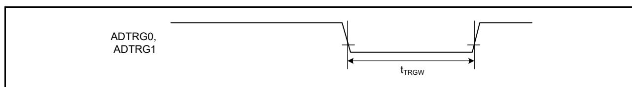
Figure 2.25 ADC12 trigger input timing
