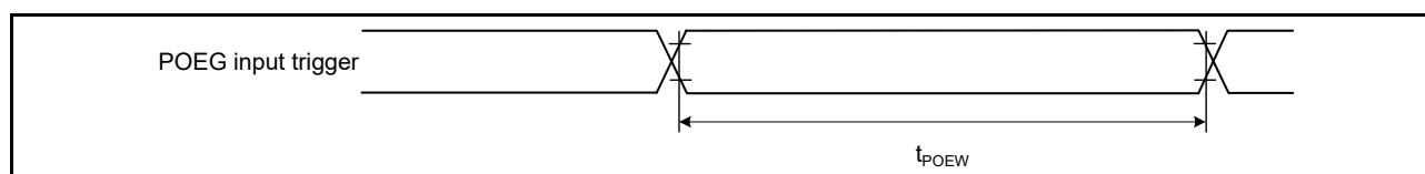
Figure 2.19 POEG input trigger timing
