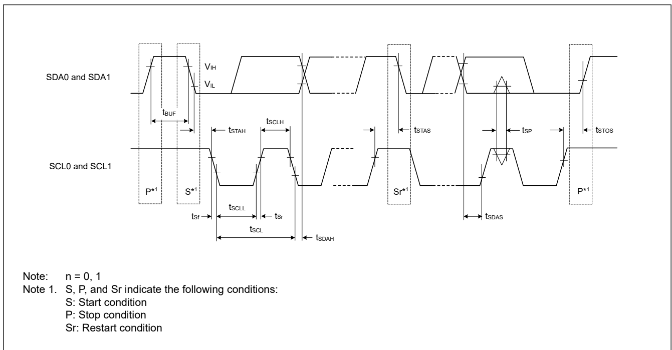
Figure 2.35 I²C bus interface input/output timing
