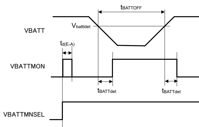
Figure 2.61 Battery backup function characteristics
