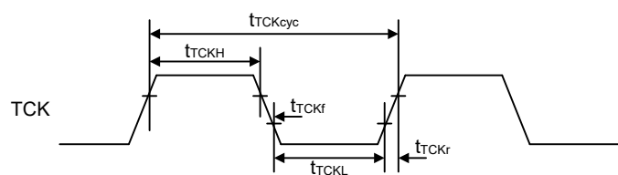
Figure 2.63 Boundary scan TCK timing
