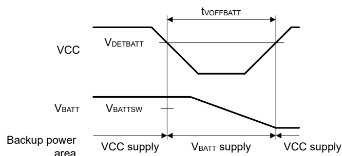
Figure 2.60 Battery backup function characteristics
