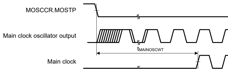
Figure 2.8 Main clock oscillation start timing
