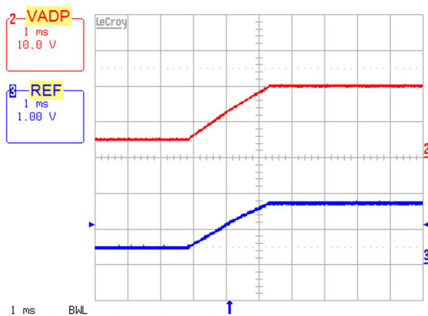
Figure 9. Reverse Mode, 5V ADP to 20V ADP
