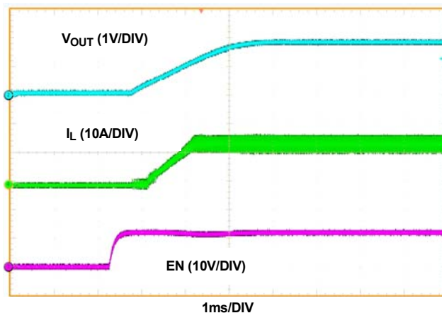
FIGURE 9. START-UP WITH EN, I_{OUT} = 14A
