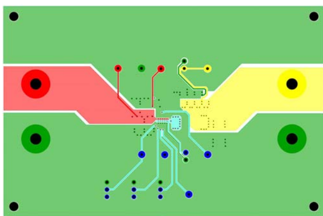
FIGURE 6. LAYER 3
