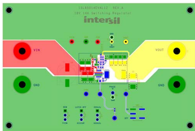
FIGURE 4. TOP LAYER
