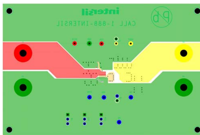
FIGURE 7. BOTTOM LAYER
