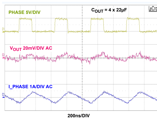
FIGURE 32. STEADY STATE AT NO LOAD ( \text{SYNC} = V_{DD} )
