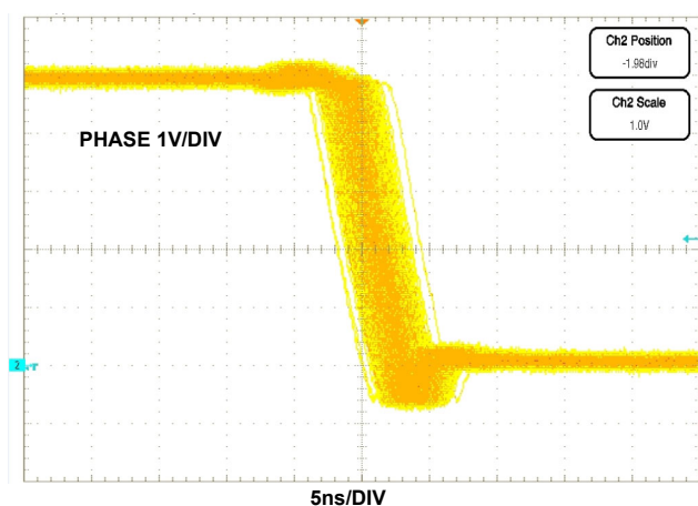
FIGURE 29. JITTER AT NO LOAD ( \text{SYNC} = V_{DD} )
