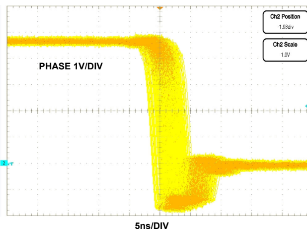
FIGURE 30. JITTER AT 5A LOAD ( \text{SYNC} = V_{DD} )
