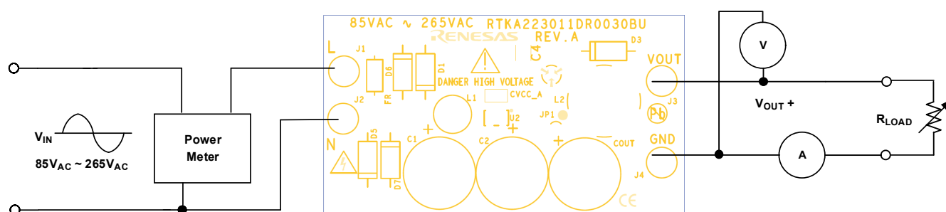
Figure 1. RTKA223011DR0030BU Connection Diagram
