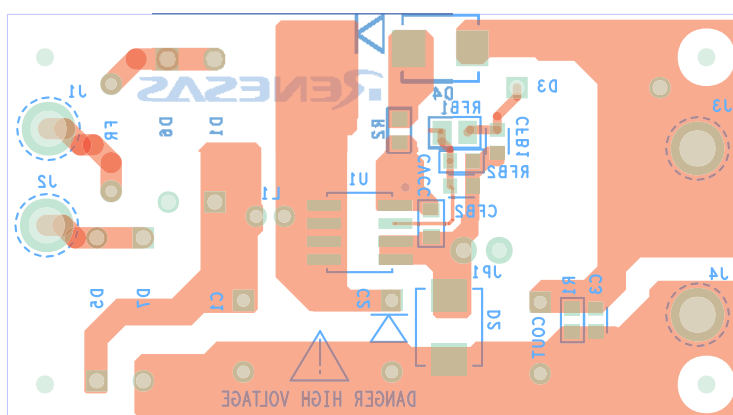
Figure 6. Bottom Layer
