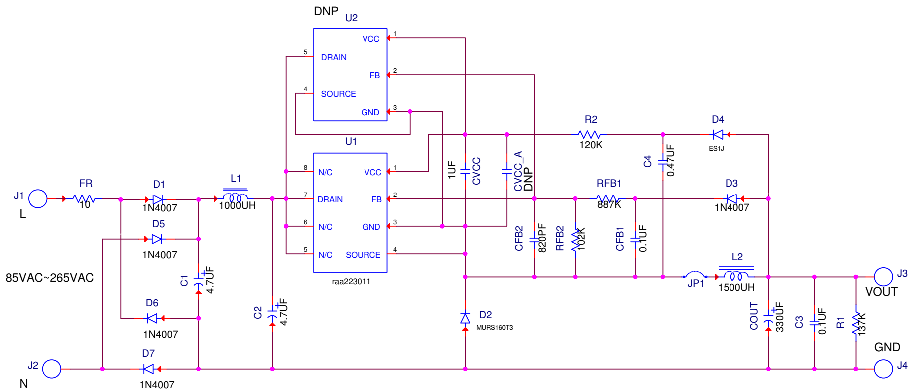
Figure 4. RTKA223011DR0030BU Schematic
