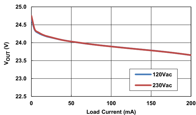
Figure 8. Load Regulation
