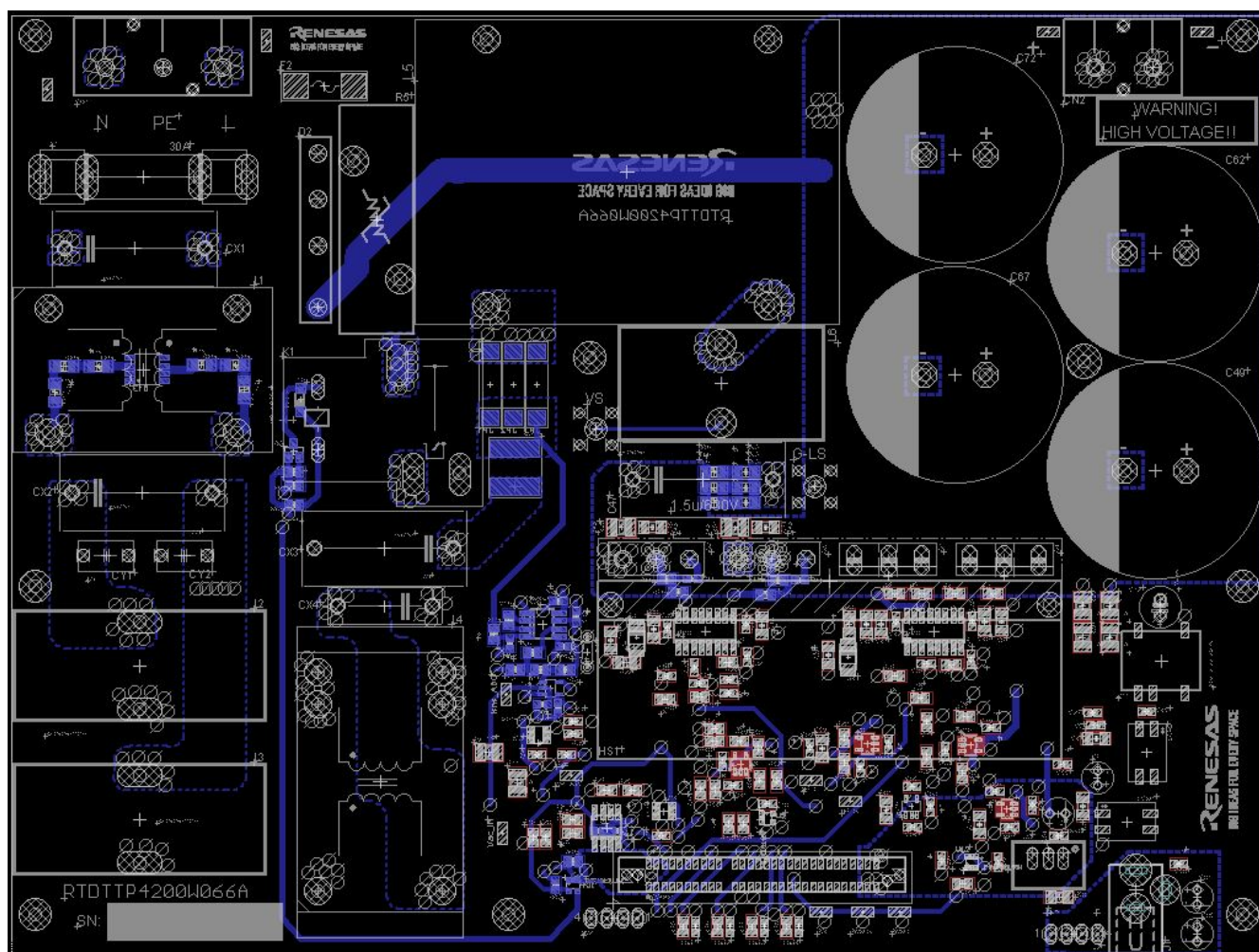
Figure 19. RTDTTP4200W066A Board – Bottom Layer
