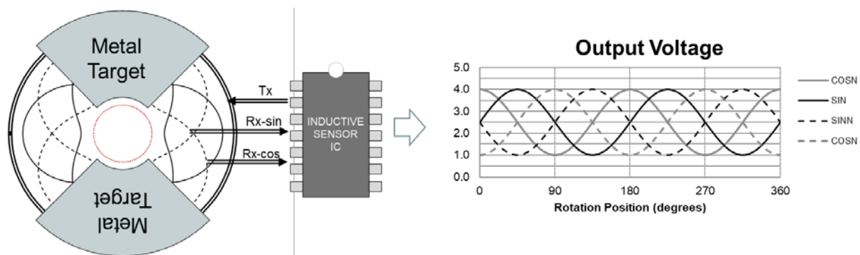
Figure 22. Coil Design and Signal Output for a 2 \times 180^\circ Rotary Sensor
