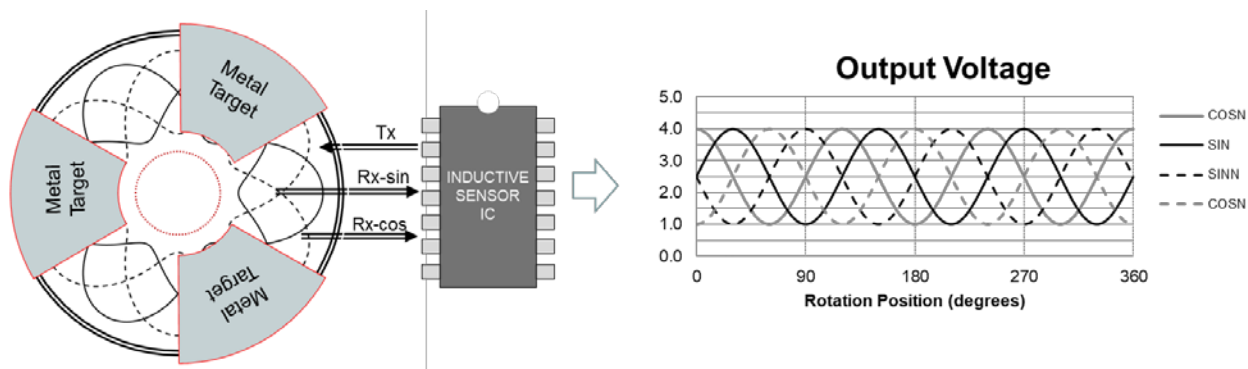
Figure 23. Coil Design and Signal Output for a 3 \times 120^\circ Rotary Sensor
