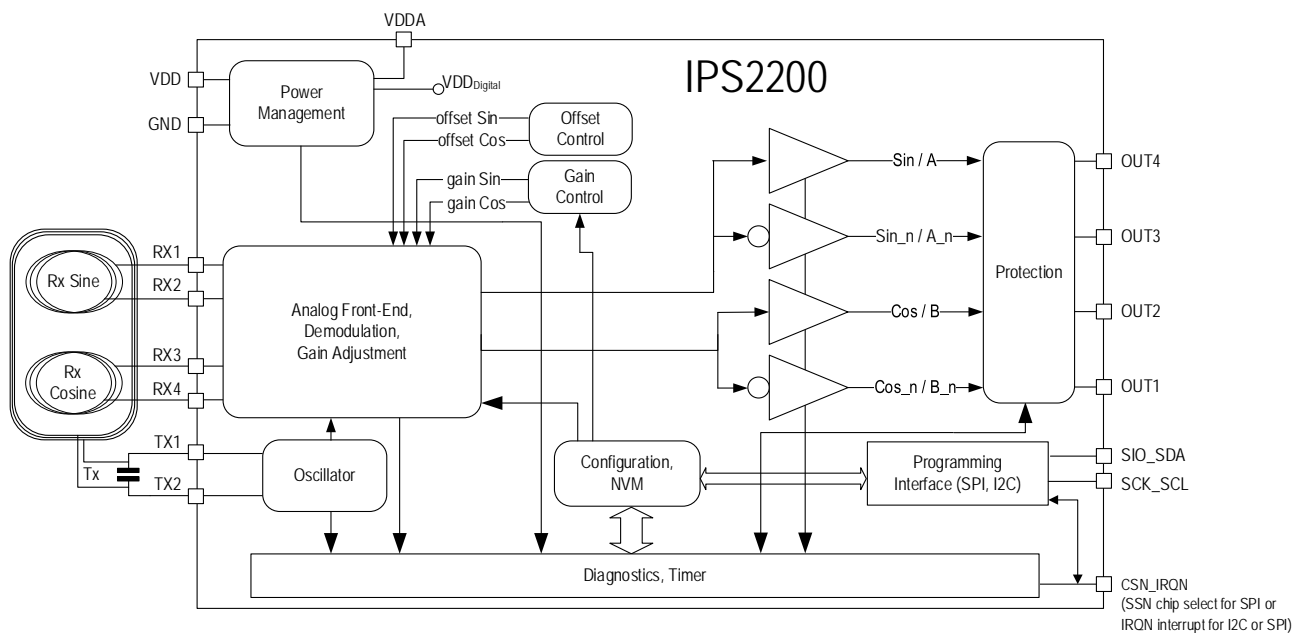
Figure 12. Block Diagram
