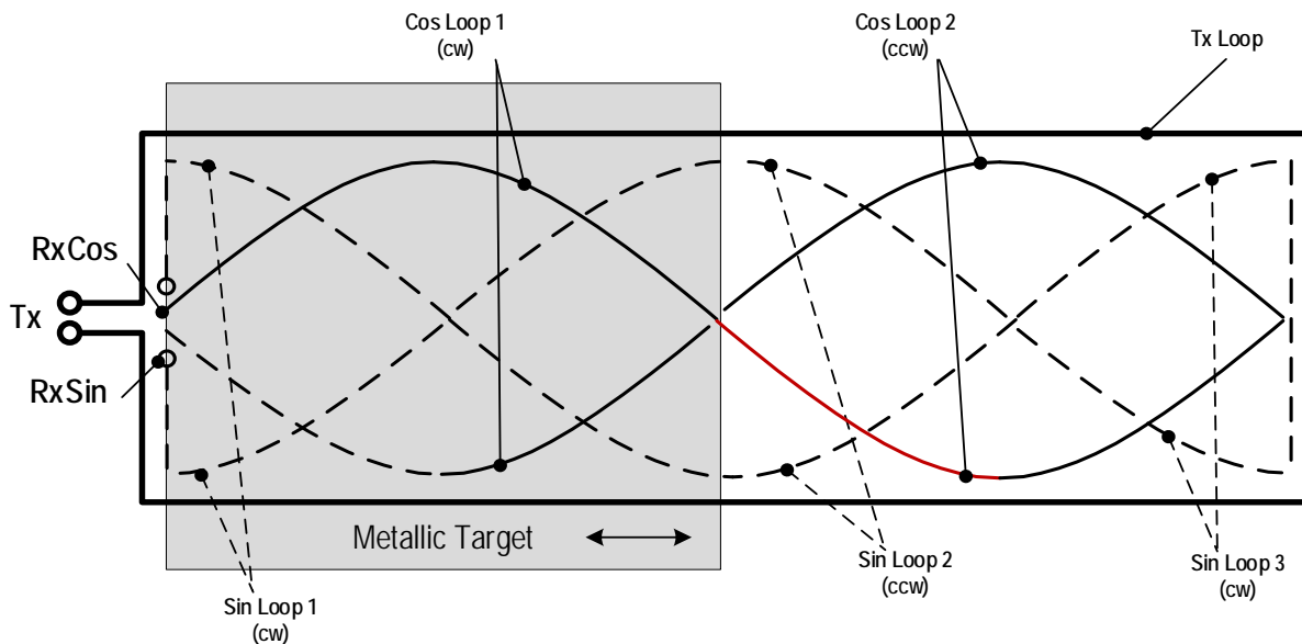
Figure 6. Coil Design for a Linear Motion Sensor
