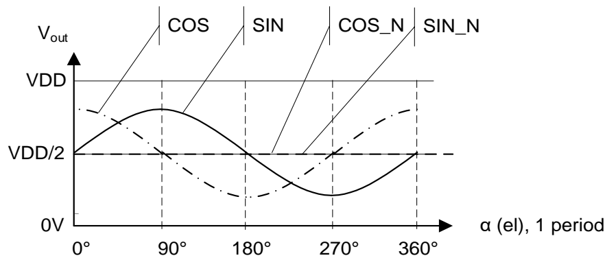
Figure 10. Sine-Cosine Analog Mode Output Signals
