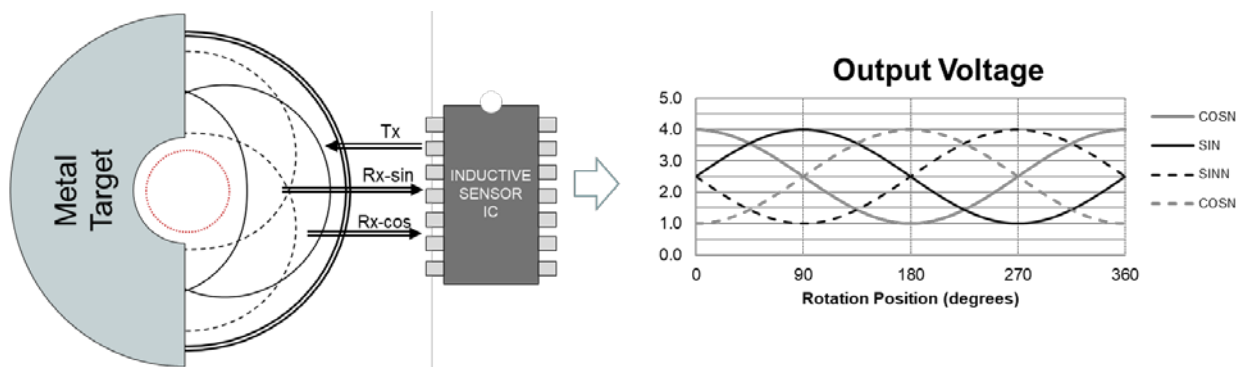
Figure 21. Coil Design and Signal Output for a 360° Rotary Sensor
