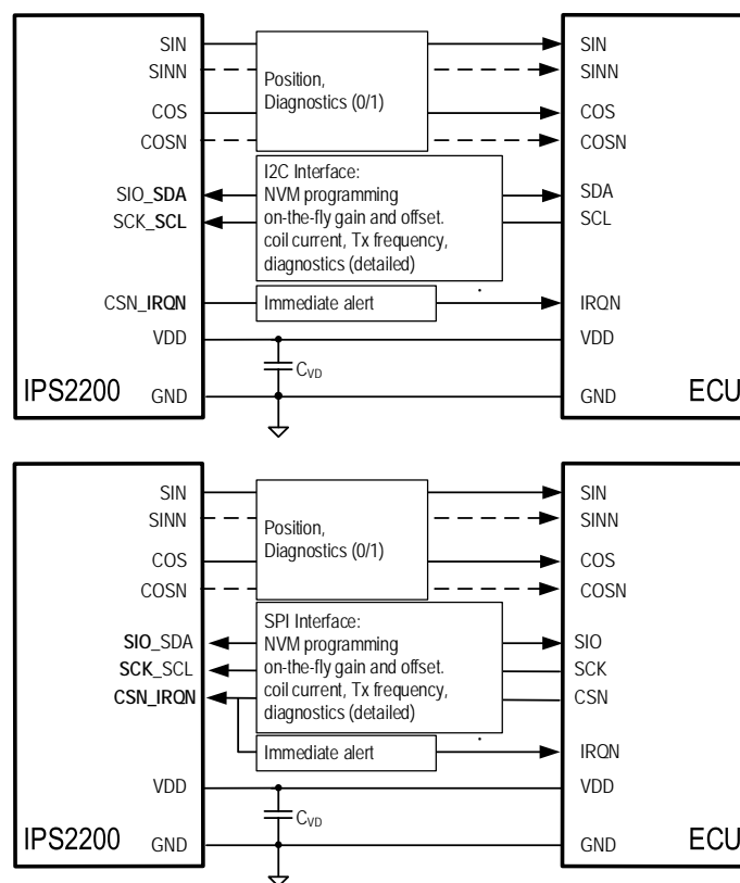
Figure 15. Analog and Digital Interface, On-The-Fly Gain and Offset Correction, Extended Diagnostics with MCU Interrupt
