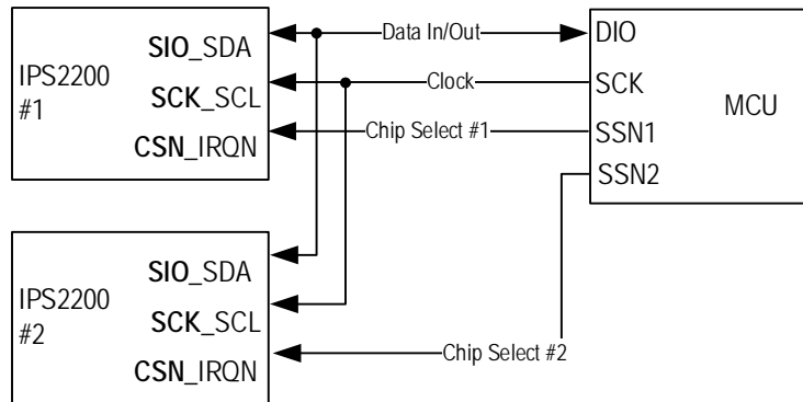
Figure 17. Half Duplex 3-3 Wire SPI Multi-slave Interface
