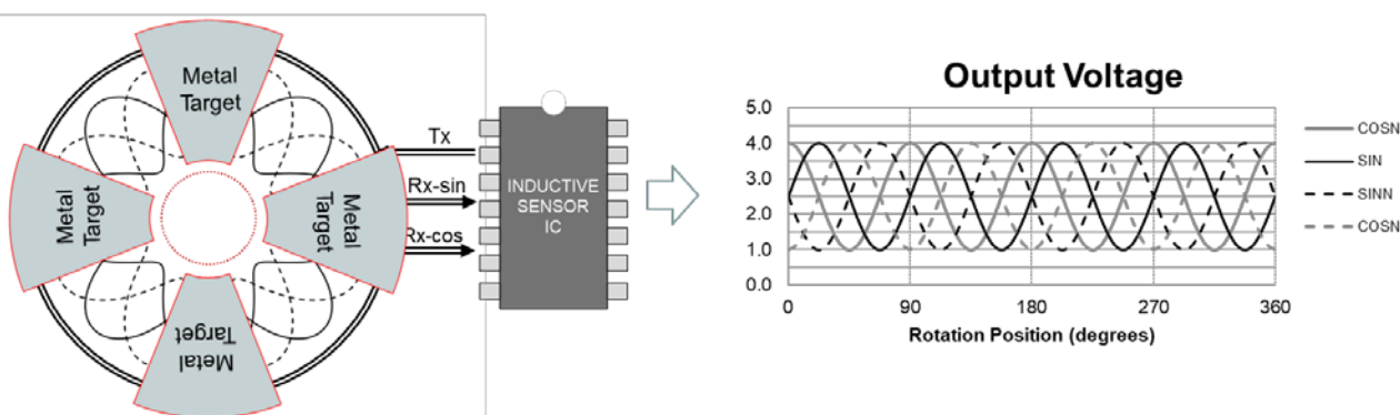
Figure 24. Coil Design and Signal Output for a 4 \times 90^\circ Rotary Sensor
