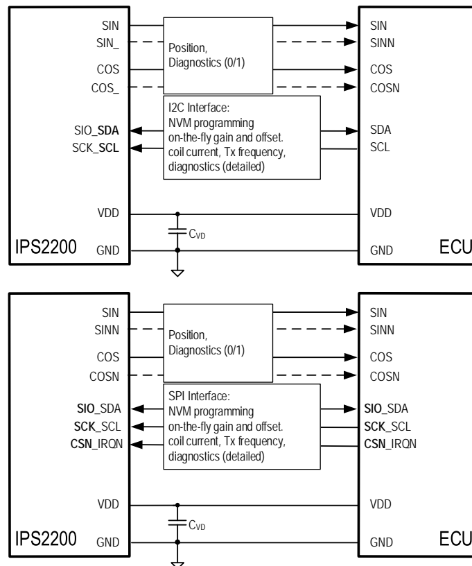
Figure 14. Analog and Digital Interface, On-The-Fly Gain and Offset Correction, Extended Diagnostics
