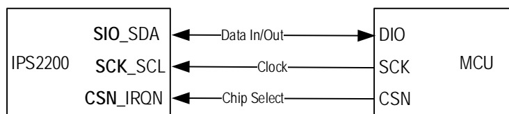
Figure 16. Half Duplex 3-3 Wire SPI Interface
