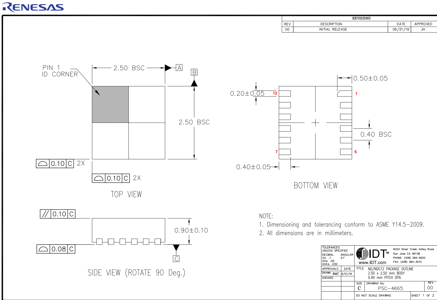
Figure 6. NDG12 Package Drawing – page 1
