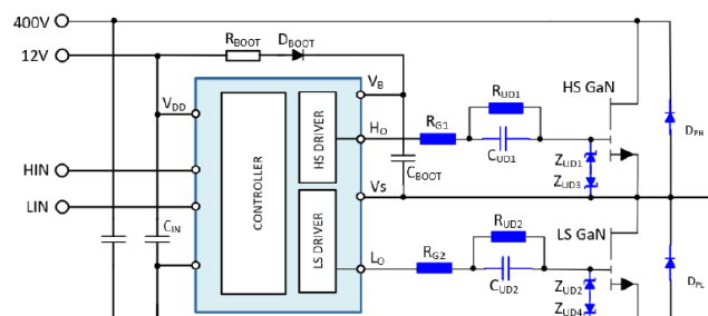
Figure 1. 1 EZDrive® GaN E-HEMT Gate Drive Circuit
