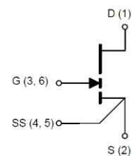
Circuit Symbol
