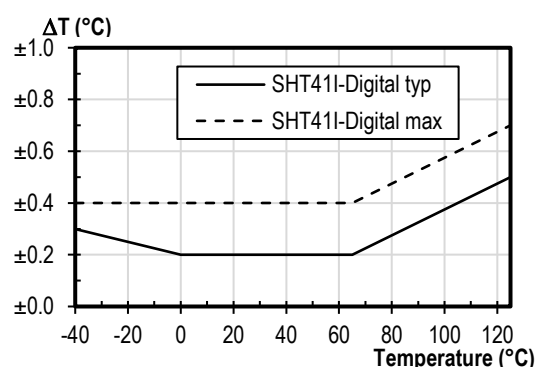
Figure 5: SHT41I-Digital typical and maximal temperature accuracy.
