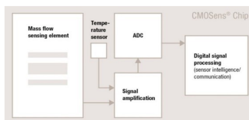
Figure 1: CMOSens® flow sensor diagram.
