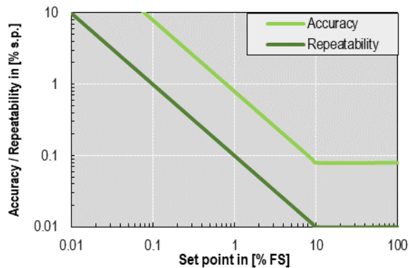
Figure 6 Accuracy and repeatability at different set points.
