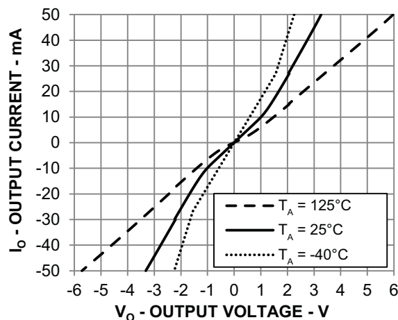
Figure 6 Output Current vs Output Voltage
