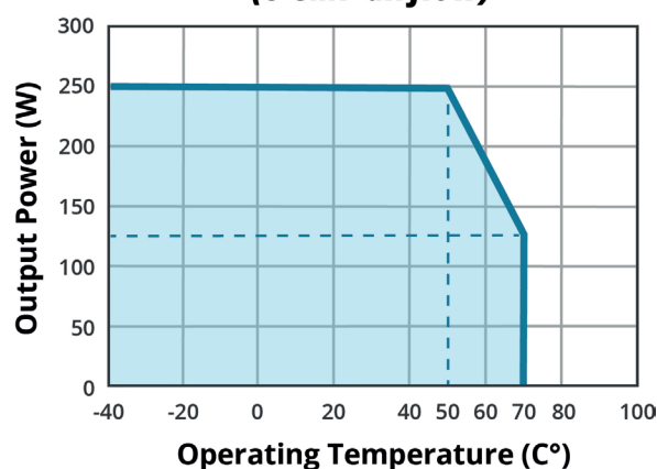
TEMPERATURE DERATING CURVE (8 CFM airflow)
