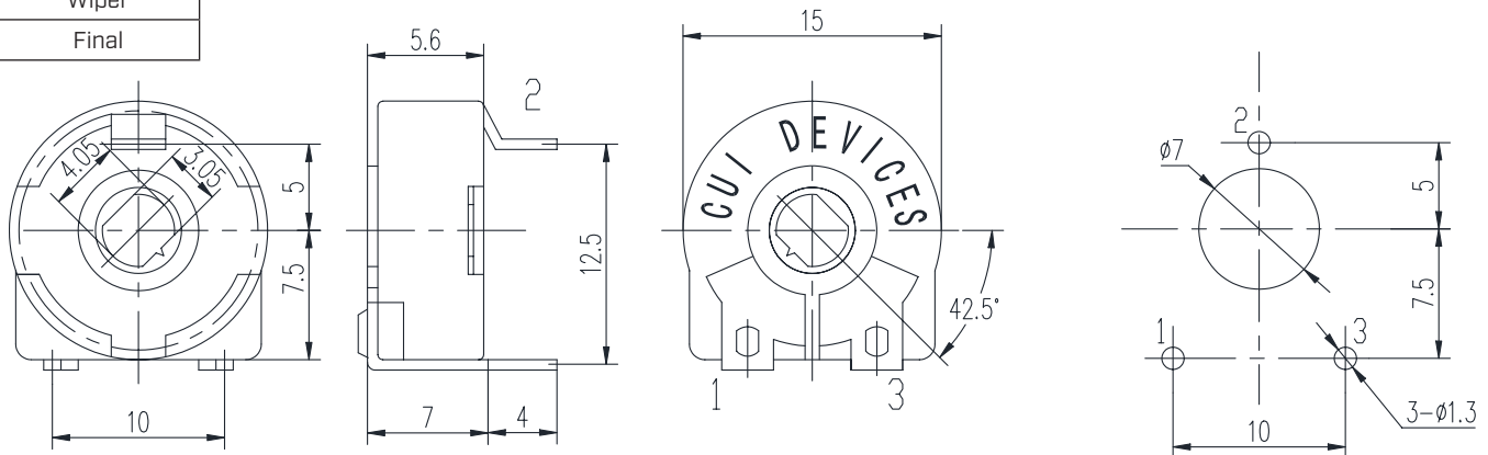
Recommended PCB Layout Top View
