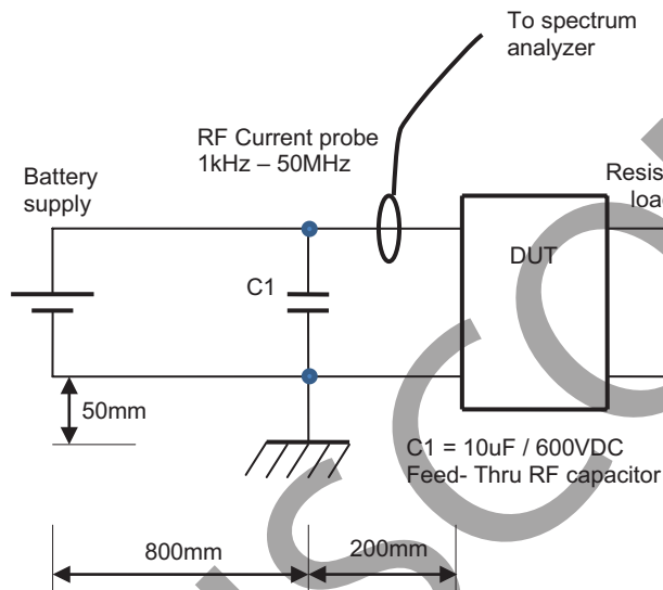
Test set-up conducted emission, power lead.
