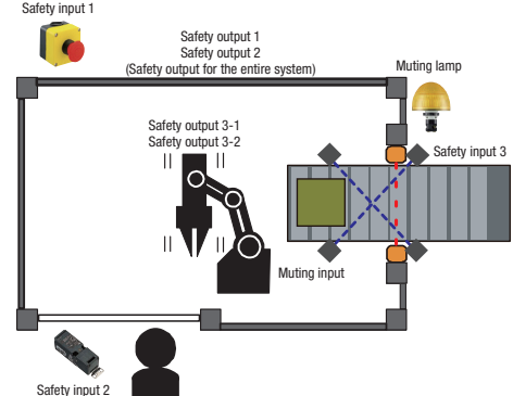
Safety system configuration example
