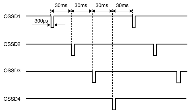
Time chart
