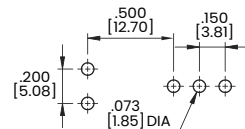
P.C.MOUNTING
