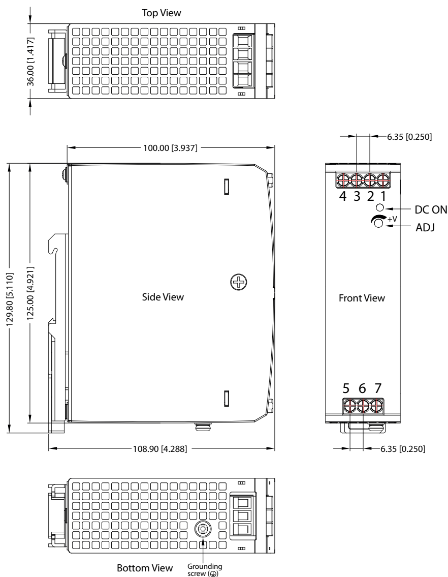
Figure 5. Mechanical Drawing
