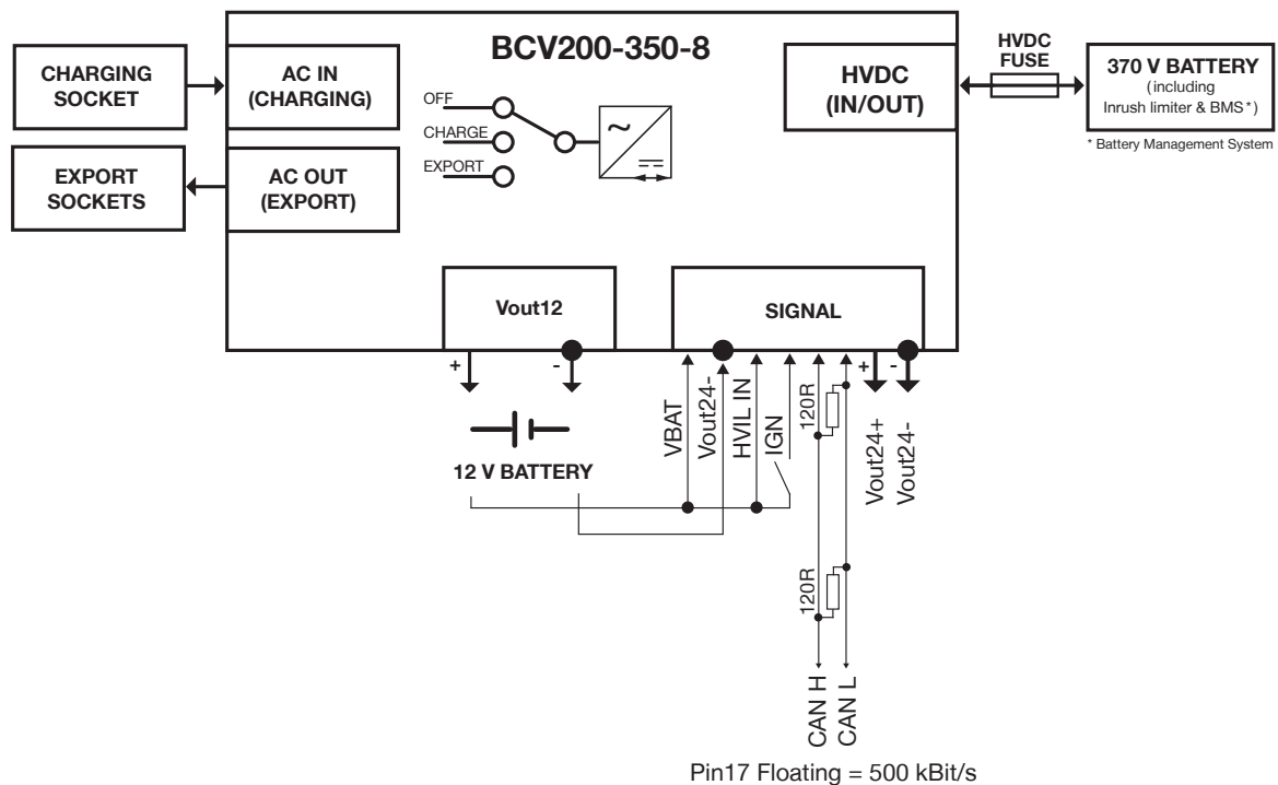
Figure 1. Schematic diagram
