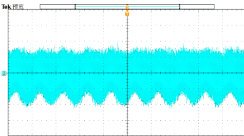
Figure 11. V_i Ripple 230VAC, full load (10ms/div)
