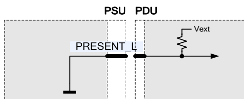
Figure 30. PRESENT_L Signal Pin
