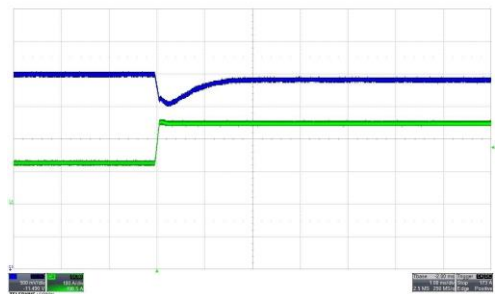
Figure 8. Load transient on V_o , 122 A to 244 A (1 ms/div) CH3 (blue): V_o (0.5 V/div), CH4 (green): I_o (100 A/div)
