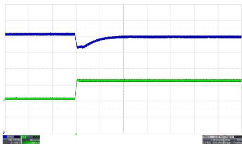
Figure 6. Load transient on V_o , 12 A to 122 A (1 ms/div) CH3 (blue): V_o (0.5 V/div), CH4 (green): I_o (100 A/div)
