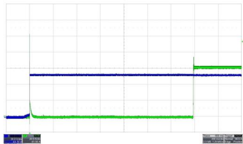
Figure 10. Inrush current, V_i = V_{i-nom} , I_i = I_{i-nom} (200 ms/div) CH3 (blue): V_i (20 V/div), CH4 (green): I_{in} (20 A/div)
