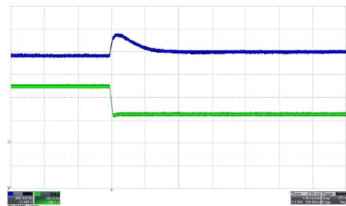
Figure 9. Load transient on V_o , 244 A to 122 A (1 ms/div) CH3 (blue): V_o (0.5 V/div), CH4 (green): I_o (100 A/div)
