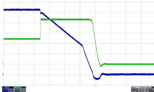
Figure 11. Short circuit on main output (500 \mu s/div) CH3 (blue): V_o (2 V/div), CH4 (green): I_o (100 A/div)
