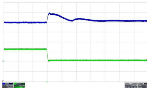
Figure 7. Load transient on V_o , 122 A to 12 A (1 ms/div) CH3 (blue): V_o (0.5 V/div), CH4 (green): I_o (100 A/div)
