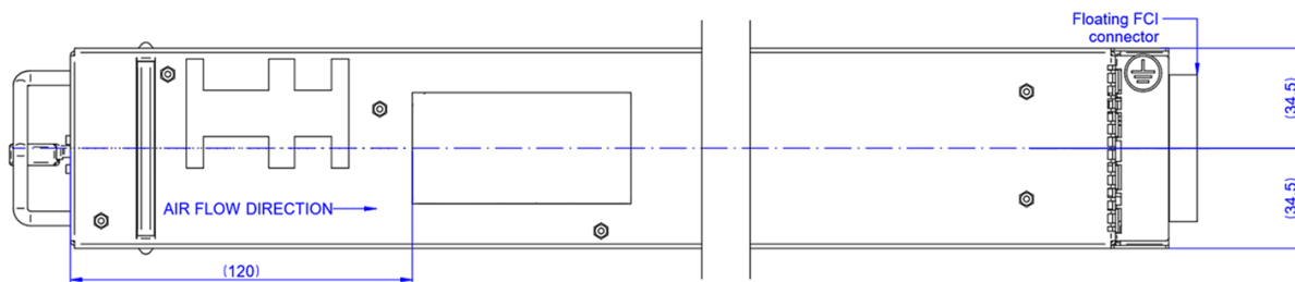
Figure 36. Top view
