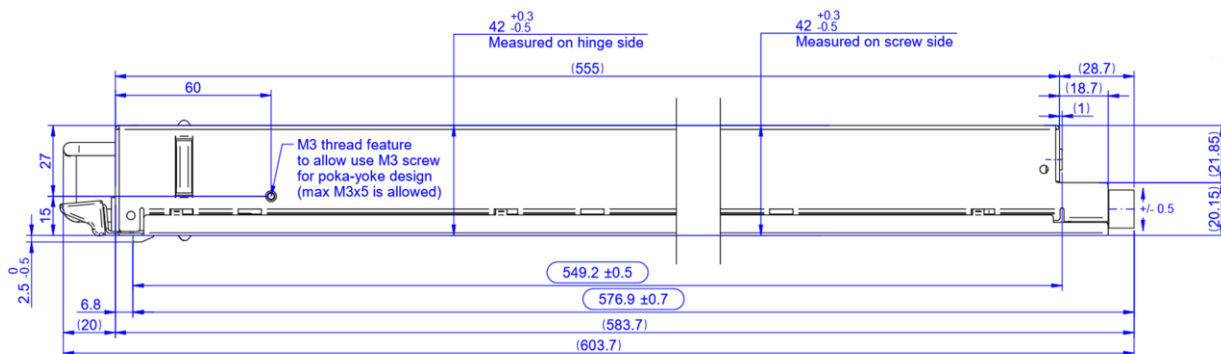
Figure 35. Side view
