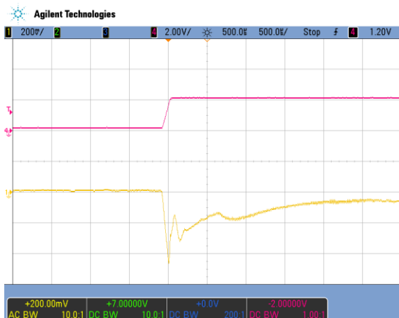
Figure 15. Load transient V1, 3 to 125 A (500 μs/div) CH1: V1 (200 mV/div); CH4: I1 (100 A/div)
