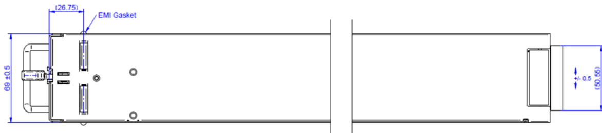
Figure 34. Bottom view
