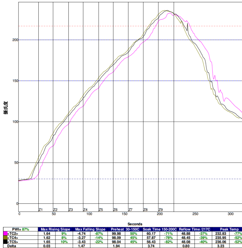
Figure 5 - Example solder reflow profile (AMW037-E03 evaluation board)
