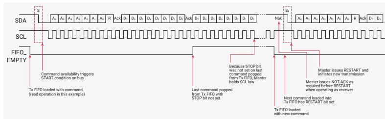
Figure 80. Master Receiver – First Command Loaded After Tx FIFO Allowed to Empty/Restart Bit Set
