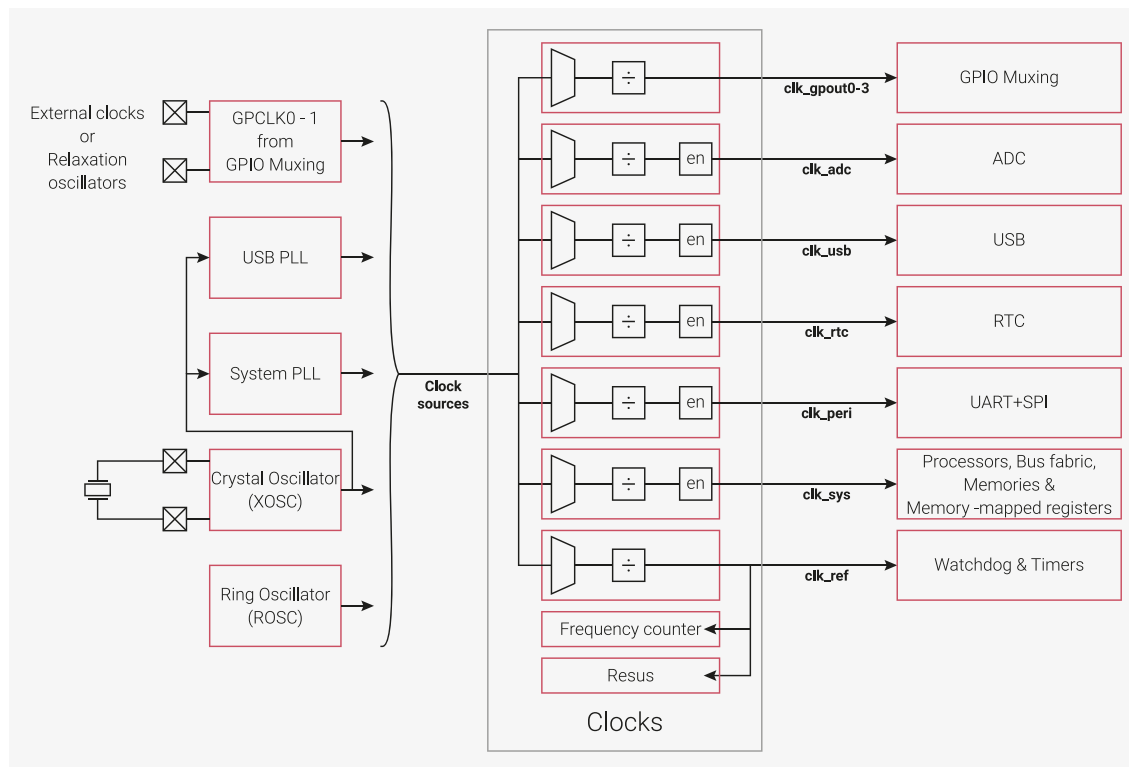
Figure 28. Clocks overview
