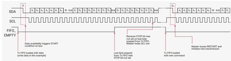
Figure 78. Master Transmitter – First Byte Loaded Into Tx FIFO Allowed to Empty, Restart Bit Set
