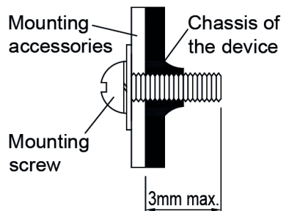
Fig. 5 Mounting Screw
