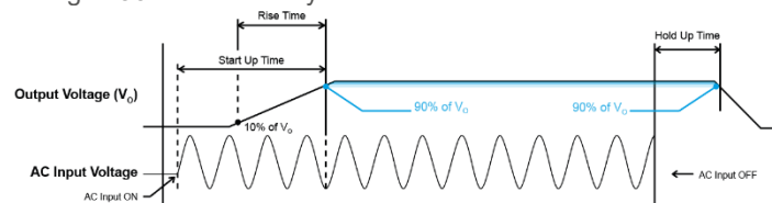
Fig. 6 Time Sequence
