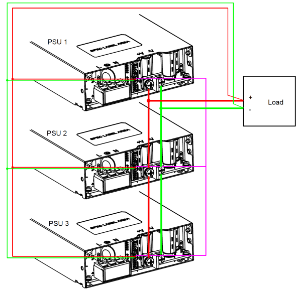
Parallel Connection with Remote Sense
