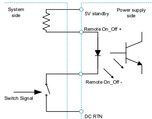
Fig. 12 Remote On_Off Connection
