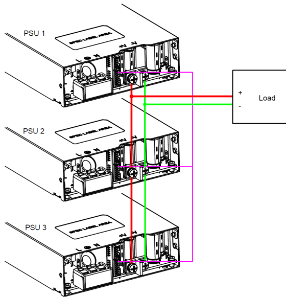
Parallel Connection without Remote Sense
