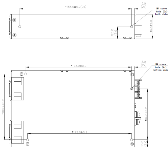
Fig. 4 Assembly Reference
