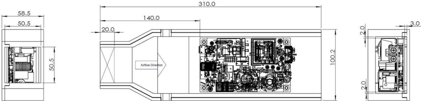
With forced airflow ( 10.873 CFM )
