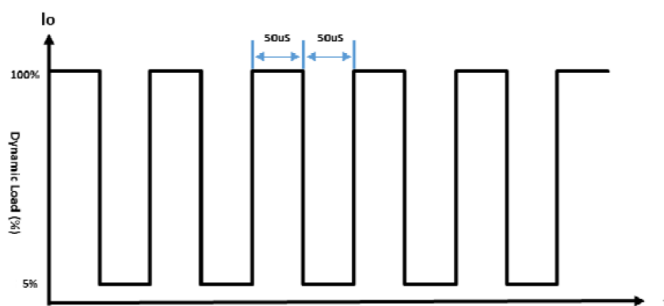
Figure 7-2. Dynamic Load (10K Hz)
