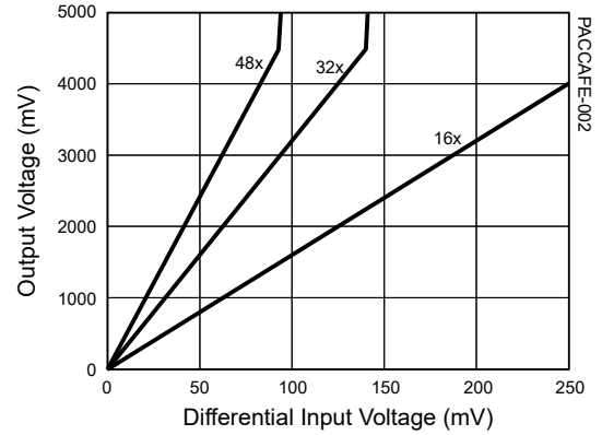
Differential PGA (DAX) Gain Characteristics at 16x, 32x, and 48x Settings
