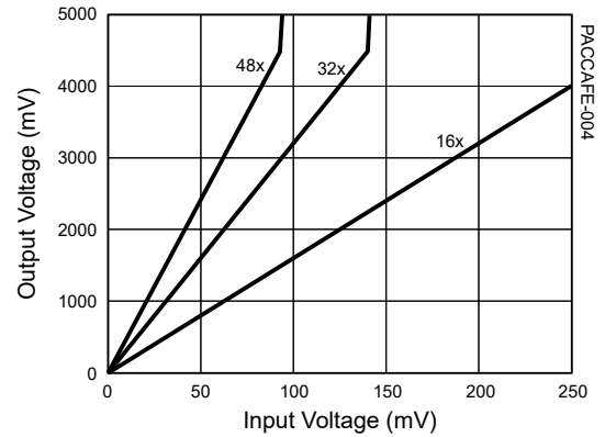
PGA (AMPx) Gain Characteristics at 16x, 32x, and 48x Settings
