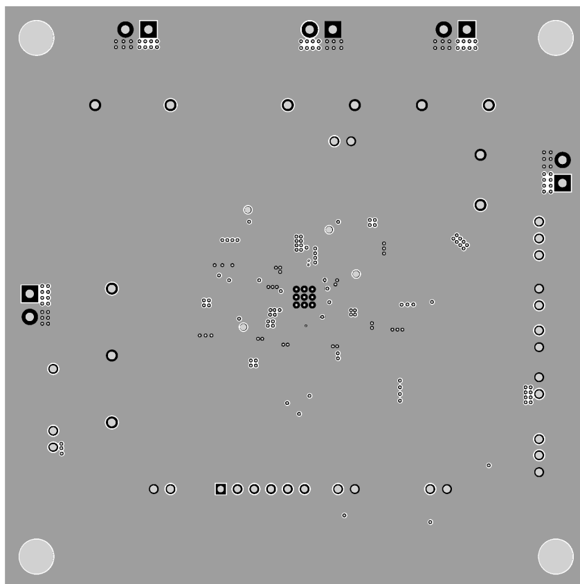
Figure 8 – Layout Layer 2
