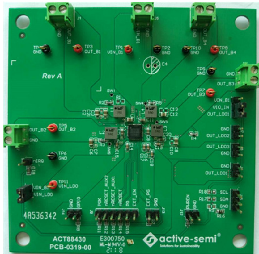
Figure 1 – EVK Picture
