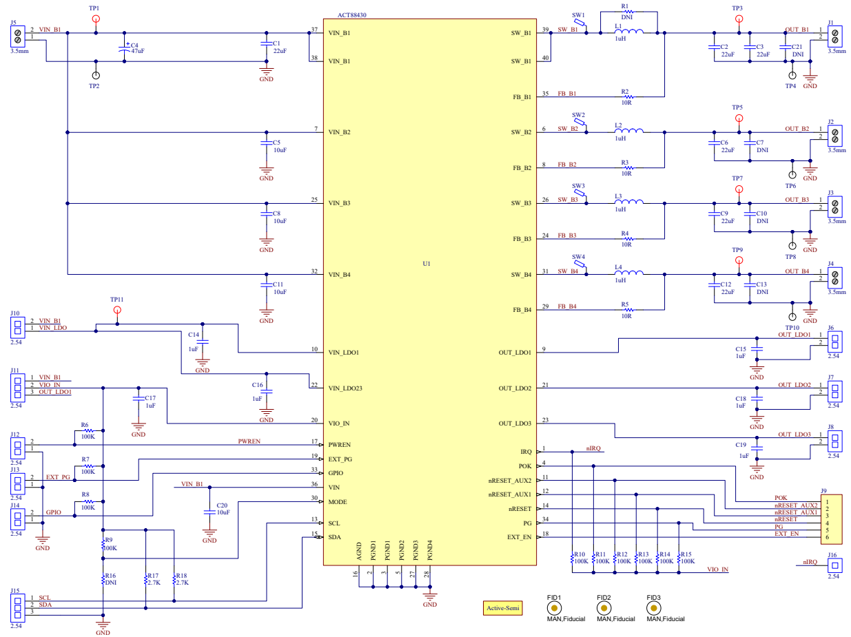
Figure 5 – ACT88430EVK1-101 Schematic
