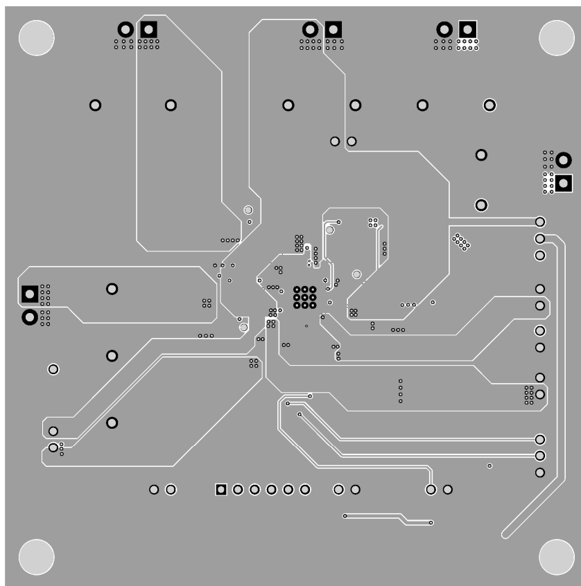
Figure 9 – Layout Layer 3
