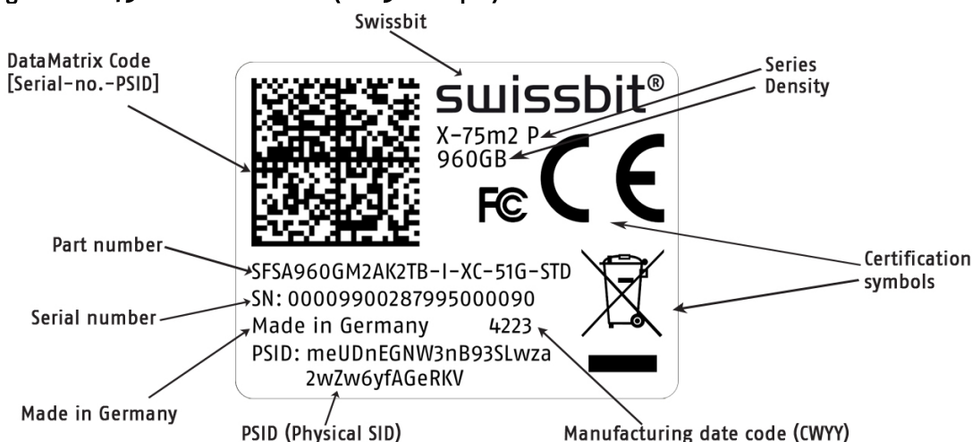
Figure 8: X-75m2 P label details (Gen5 example)
