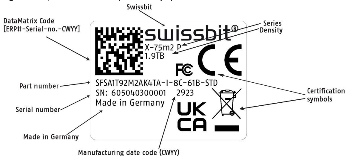
Figure 7: X-75m2 P label details (Gen4 example)
