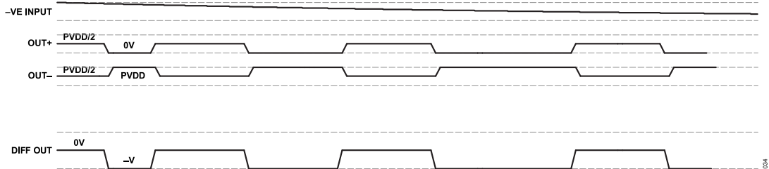
Figure 34. Negative Output, Three-Level, \Sigma - \Delta Output Modulation
