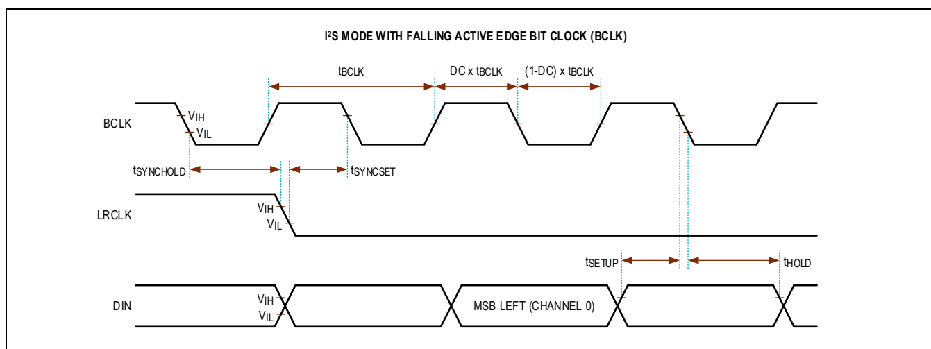
Figure 2. PCM Interface Timing Diagram for I^2S Mode
