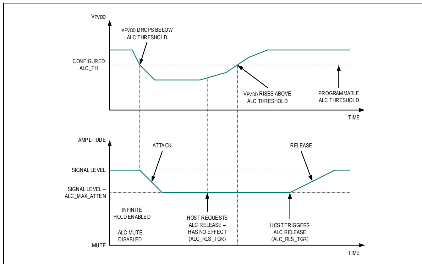
Figure 24. Brownout Protection ALC with Infinite Hold Enabled and Mute Disabled
