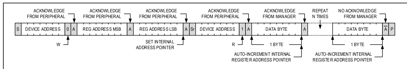
Figure 18. I 2 C Manager Reading n-Bytes of Data from the Peripheral Device
