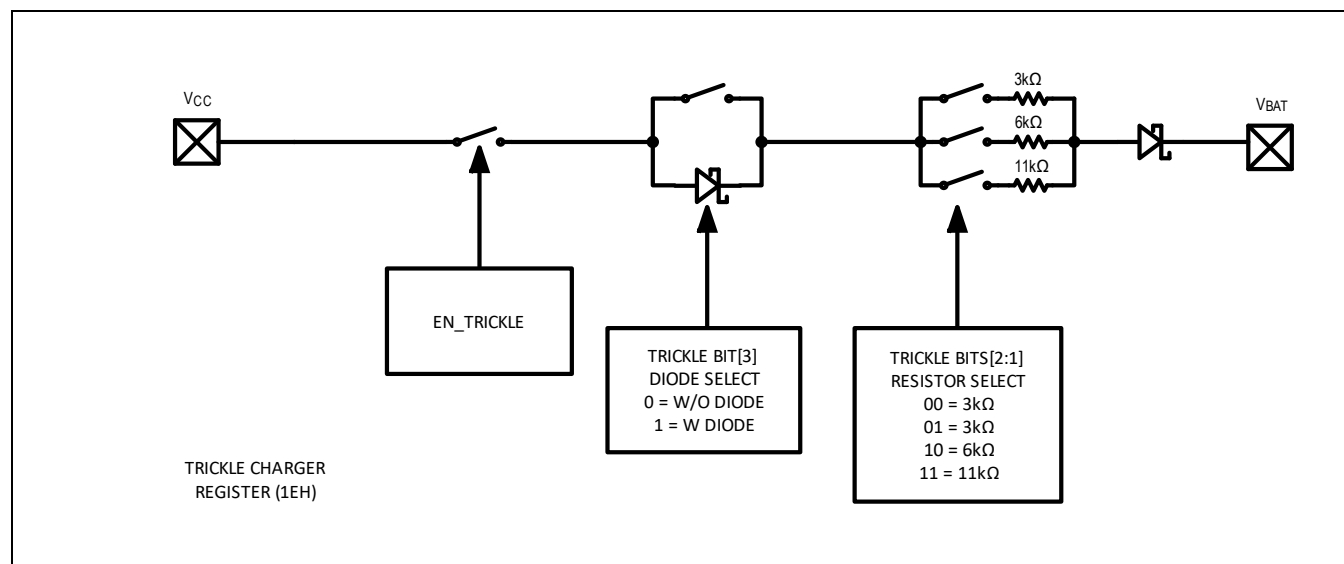
Figure 3. Trickle Charger
