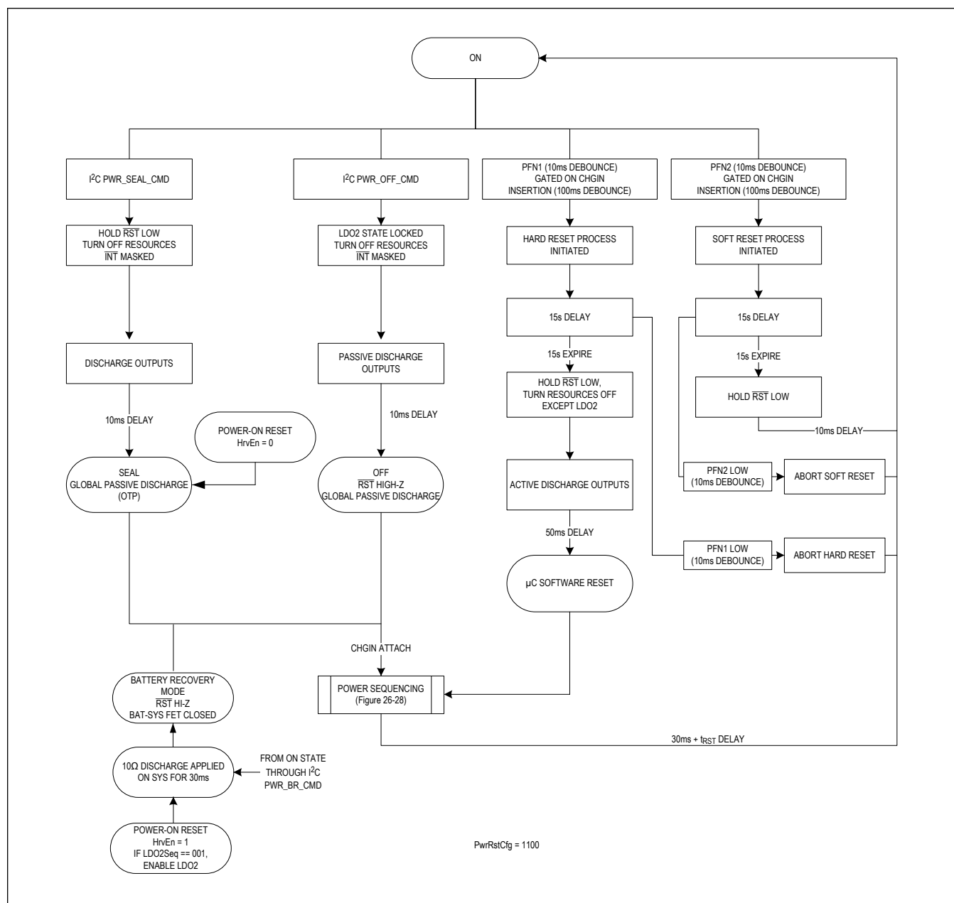
Figure 23. PwrRstCfg 1100
