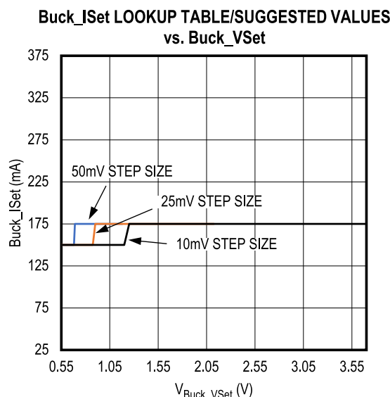
Figure 14. Optimal Peak Current Setting vs. Output Voltage
