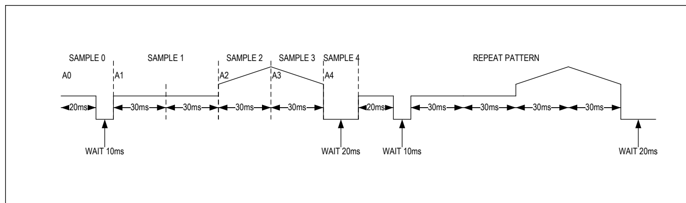
Figure 35. Diagram of Haptic Driver Output for Sample Pattern Stored Pattern
