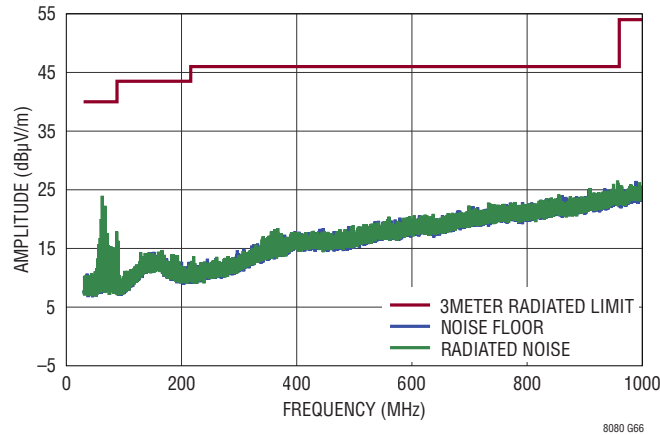
DC3071A DEMO BOARD V_{\text{IN}} = 24\text{V} , V_{\text{OUT1/2}} = 3.3\text{V} , I_{\text{OUT1/2}} = 500\text{mA}
