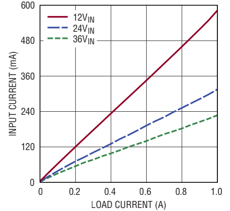
I_{\text{IN}} vs I_{\text{OUT}} , V_{\text{OUT}} = 5\text{V} , V_{\text{OUT1,2}} in Parallel, Burst-Mode Operation
