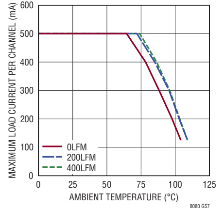
Thermal Derating 24V IN to 5V OUT , I_{\text{BUS}} = I_{\text{OUT1,2}} = 0.5\text{A} DC3071A Demo Board
