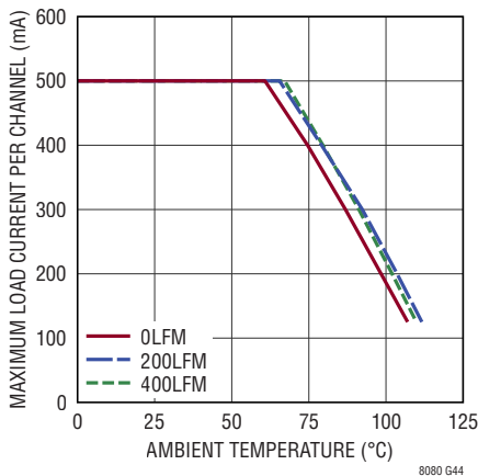
Thermal Derating 12V_{\text{IN}} to 1.2V_{\text{OUT}} , V_{\text{BUS}} = 2.5\text{V} , I_{\text{BUS}} = I_{\text{OUT1,2}} = 0.5\text{A} DC3071A Demo Board
