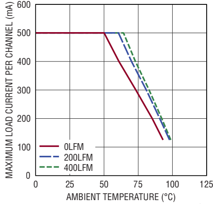
Thermal Derating 36\text{V}_{\text{IN}} to 8\text{V}_{\text{OUT}} , I_{\text{BUS}} = 0\text{A} , I_{\text{OUT1,2}} = 0.5\text{A} DC3071A Demo Board
