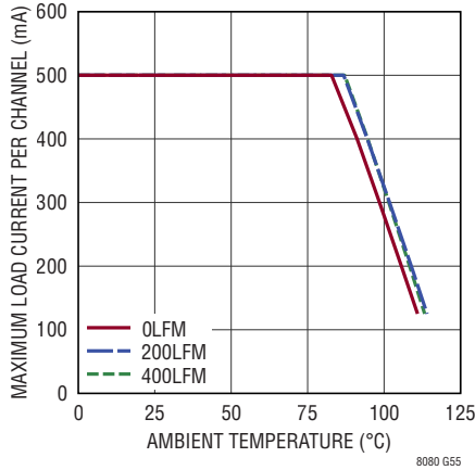
Thermal Derating 36V IN to 3.3V OUT , I_{\text{BUS}} = I_{\text{OUT1,2}} = 0.5\text{A} DC3071A Demo Board
