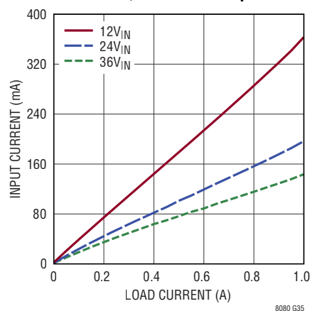
I_{\text{IN}} vs I_{\text{OUT}} , V_{\text{OUT}} = 2.5\text{V} , V_{\text{OUT1,2}} in Parallel, Burst-Mode Operation
