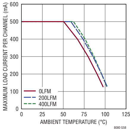
Thermal Derating 36V IN to 5V OUT , I_{\text{BUS}} = I_{\text{OUT1,2}} = 0.5\text{A} DC3071A Demo Board
