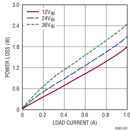
Power Loss, V_{\text{OUT}} = 1.8\text{V} , V_{\text{OUT1,2}} in Parallel, Burst-Mode Operation
