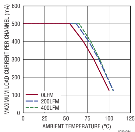
Thermal Derating 36V IN to 2.5V OUT , I BUS = I OUT1,2 = 0.5A DC3071A Demo Board
