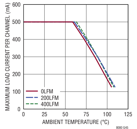
Thermal Derating 24V_{\text{IN}} to 1.2V_{\text{OUT}} , V_{\text{BUS}} = 2.5\text{V} , I_{\text{BUS}} = I_{\text{OUT1,2}} = 0.5\text{A} DC3071A Demo Board
