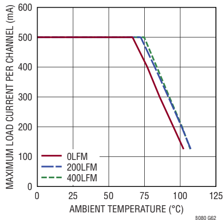
Thermal Derating 24V IN to 8V OUT , I_{\text{BUS}} = 0\text{A} , I_{\text{OUT1,2}} = 0.5\text{A} DC3071A Demo Board
