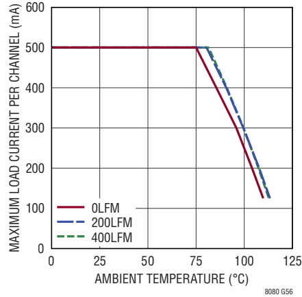
Thermal Derating 12V IN to 5V OUT , I_{\text{BUS}} = I_{\text{OUT1,2}} = 0.5\text{A} DC3071A Demo Board
