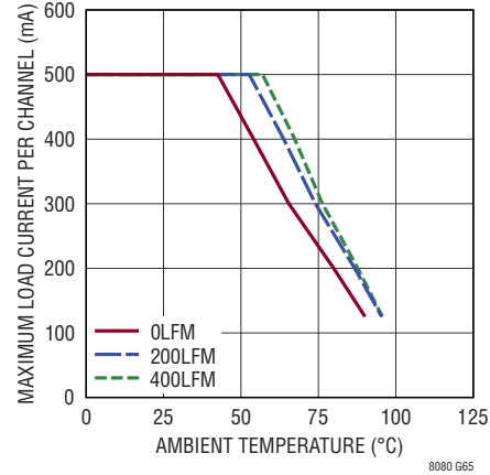
Thermal Derating 36\text{V}_{\text{IN}} to 8\text{V}_{\text{OUT}} , I_{\text{BUS}} = I_{\text{OUT1,2}} = 0.5\text{A} DC3071A Demo Board
