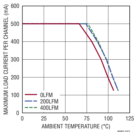
Thermal Derating 24V IN to 2.5V OUT , I BUS = I OUT1,2 = 0.5A DC3071A Demo Board
