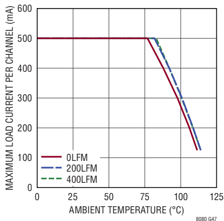
Thermal Derating 36V IN to 1.8V OUT , I BUS = I OUT1,2 = 0.5A DC3071A Demo Board
