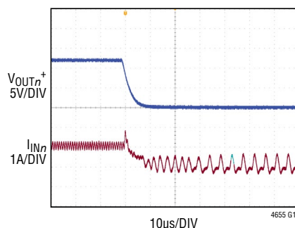
Short Circuit, 4A Load
