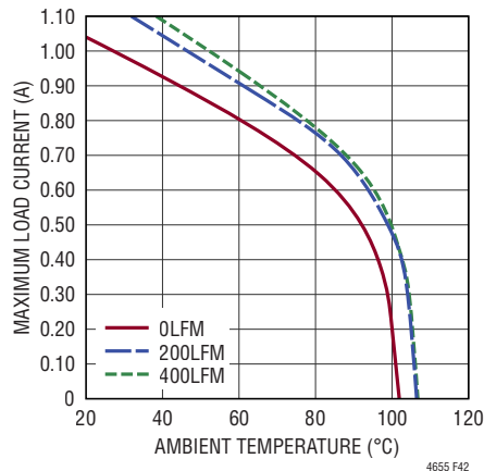
Figure 42. 5V to -24V_{OUT} Derating Curve, with BGA Heat Sink
