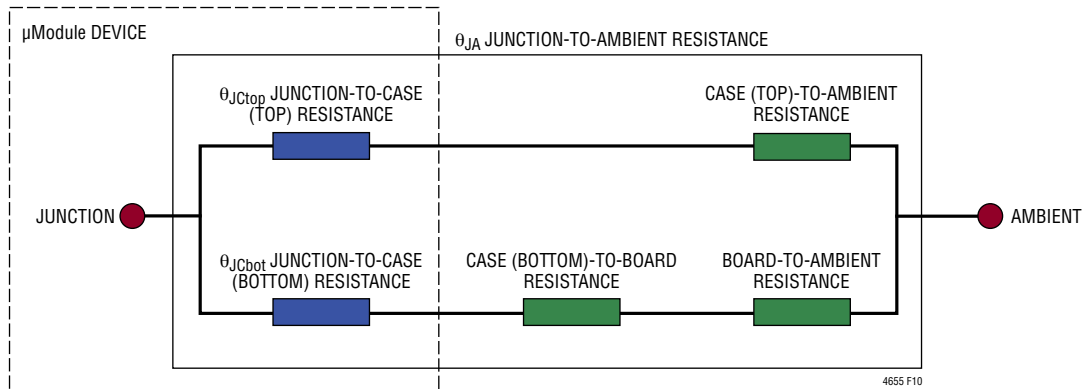
Figure 10. Graphical Representation of JESD51-12 Thermal Coefficients
