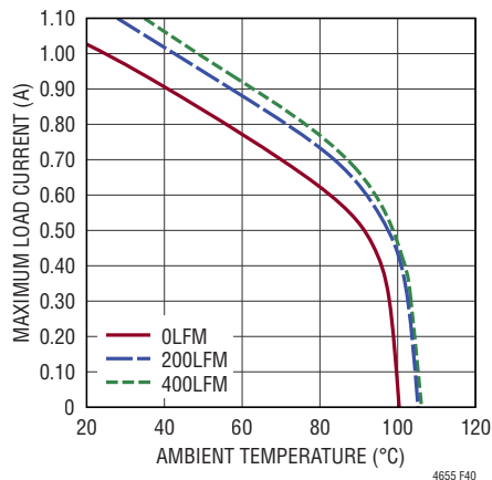
Figure 40. 5V to -24V_{OUT} Derating Curve, No Heat Sink
