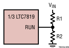
Figure 5. Using the RUN Pins As a UVLD
