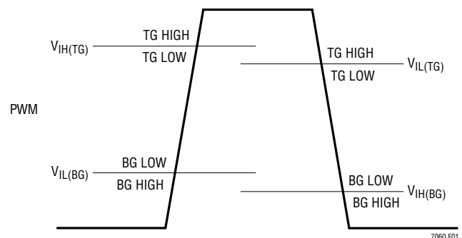
Figure 1. Three-State PWM Operation
