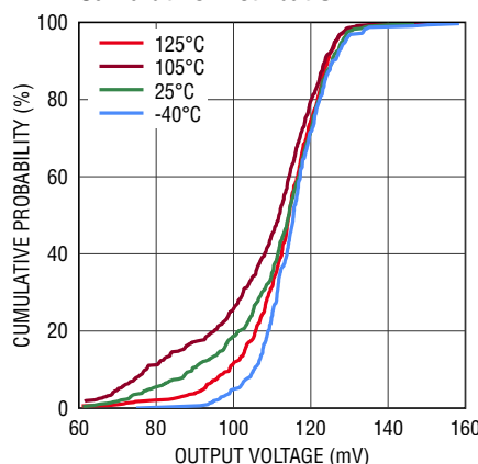
Output Voltage at -35dBm Cumulative Distribution
