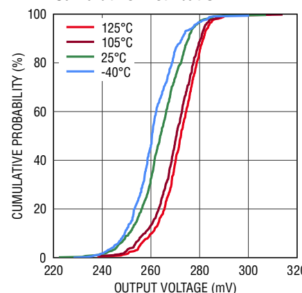
Output Voltage at -30dBm Cumulative Distribution
