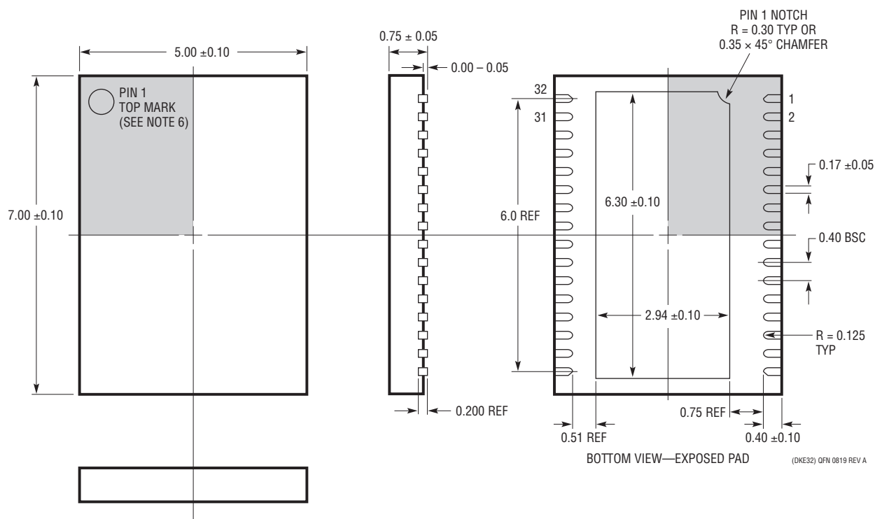
DKE Package 32-Lead Plastic DFN (7mm × 5mm) (Reference LTC DWG # 05-08-1789 Rev A)
