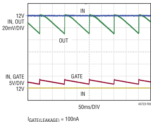
Figure 3. Regulating \Delta V_{SD} at Low I_{\text{LOAD}} = 1\mu\text{A}
