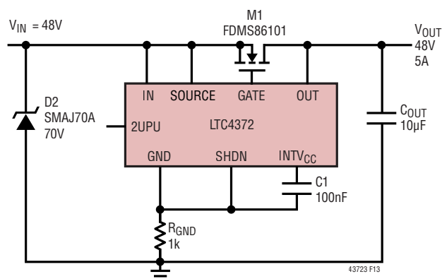
Figure 13. 48V Ideal Diode without Reverse Input Protection
