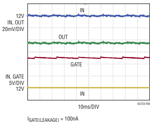
Figure 5. Regulating \Delta V_{SD} at High I_{\text{LOAD}} = 16\text{A}
