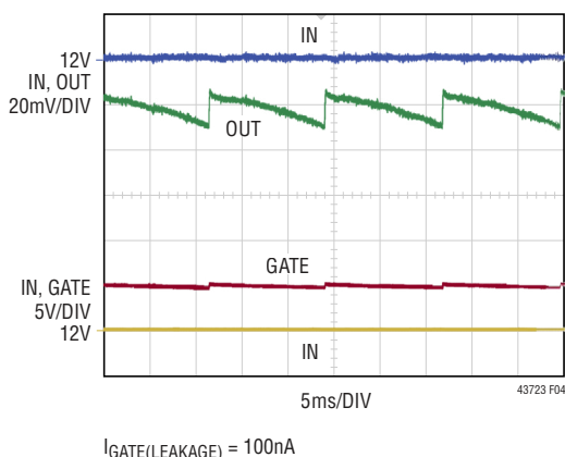
Figure 4. Regulating \Delta V_{SD} at Moderate I_{\text{LOAD}} = 2\text{A}
