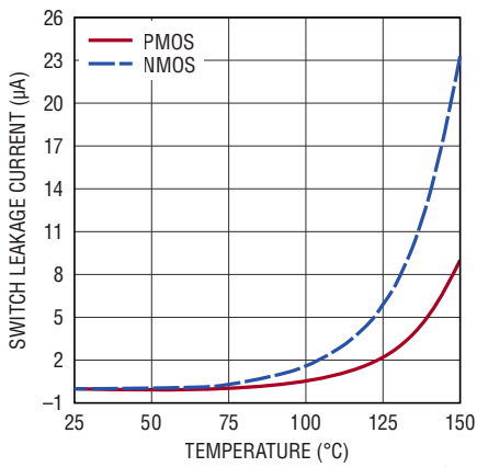
Switch Leakage
