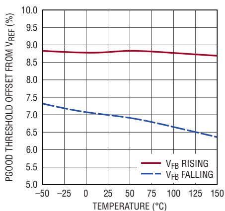
OV PGOOD Threshold
