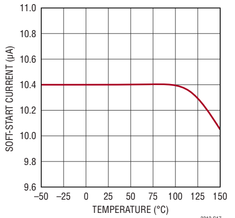
Soft-Start Current
