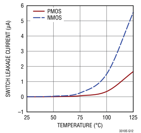
Switch Leakage
